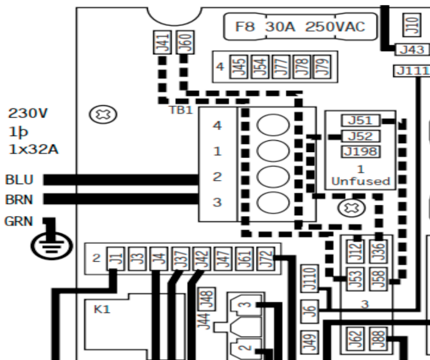
Cablage monophasé (1 x 16amps/32amps)
